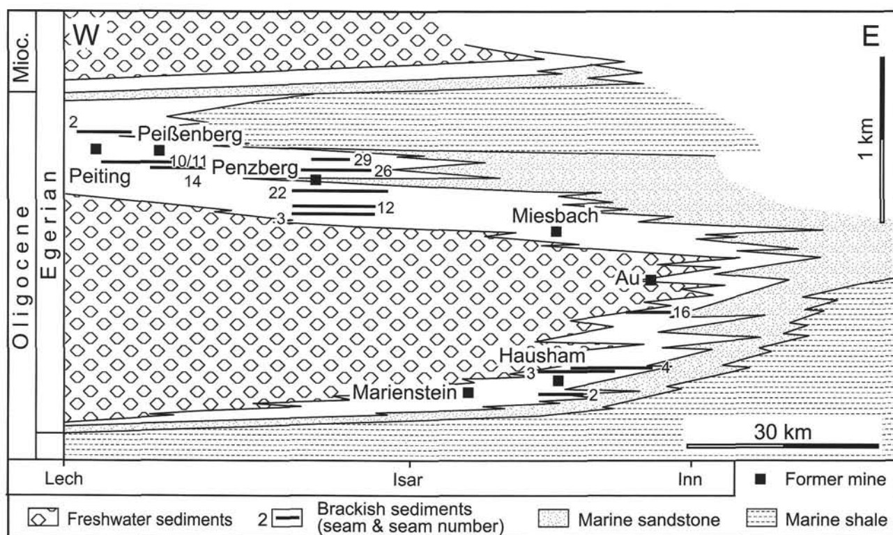
Fig. 3 Schematic W-E cross-section through the Upper Bavarian coal district (modified after GEISSLER, 1975). Position of cross-section is shown in Fig. 1. Note, that positions of seams are shown only for the Hausham, Penzberg and Peiting areas. A high number of relatively thin seams is typical for foreland basins. The regional distribution of the deposits is controlled by regressions and transgressions.
